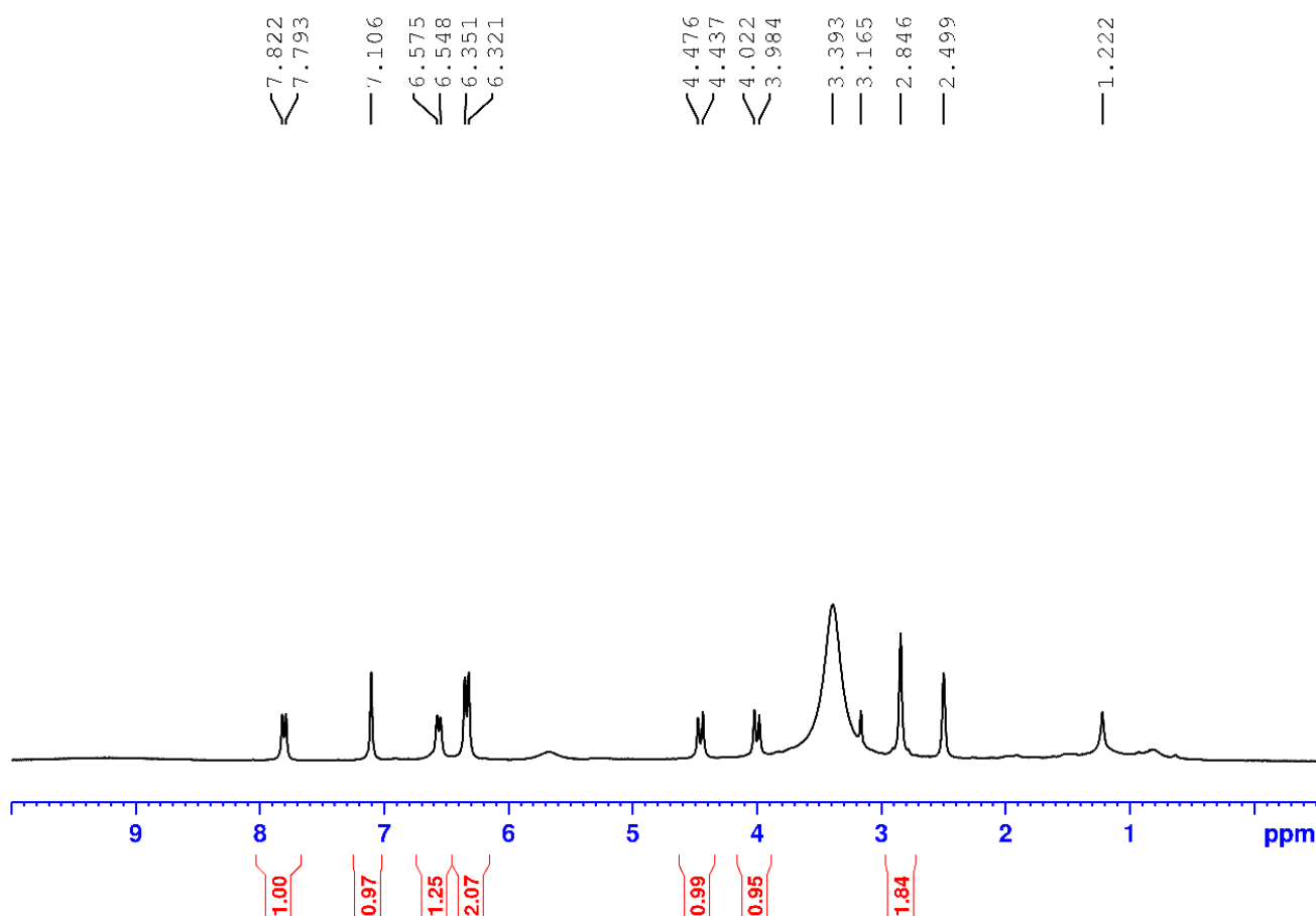
Figure S1 1 H NMR spectrum of brazilein
