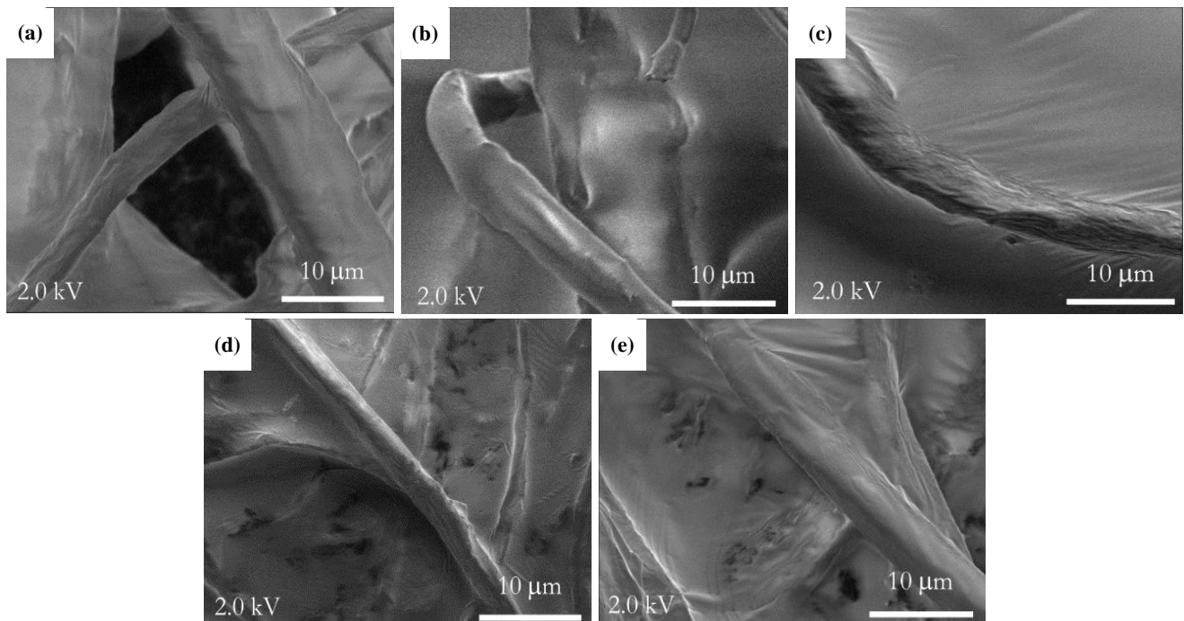
Figure S1. FE-SEM ( \times 3000 ) of the CFs/CNT all neat PU resin, (a) CFs without CNT, (b) CFs/CNT 0.5, (c) CFs/CNT 1.5, (d) CFs/CNT 2.5, (e) CFs/CNT 5.0.
